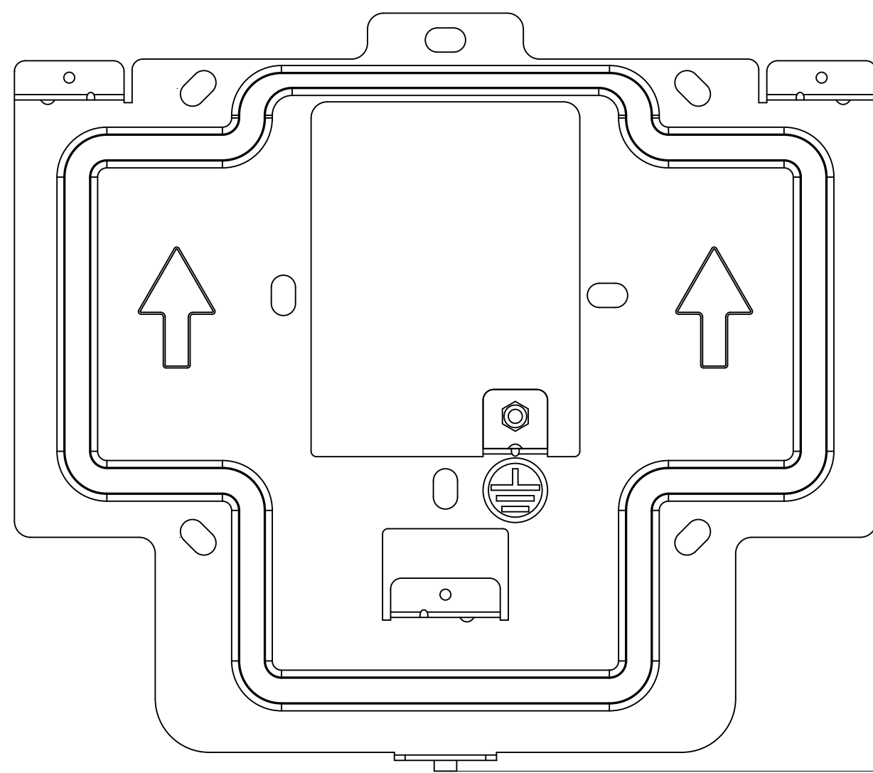
2 FRONT VIEW:WALL MOUNTING BRACKET PLACEMENT
